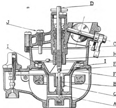
SECTION VIEW OF HOLLEY CARBURETER.
